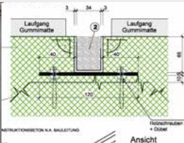
Detailpläne
